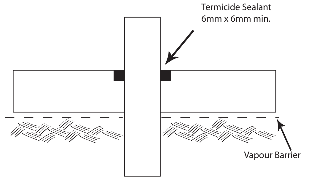
Retro Sealant Detail
