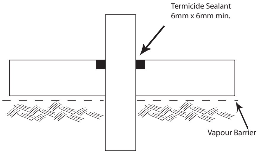
Retro Sealant Detail
